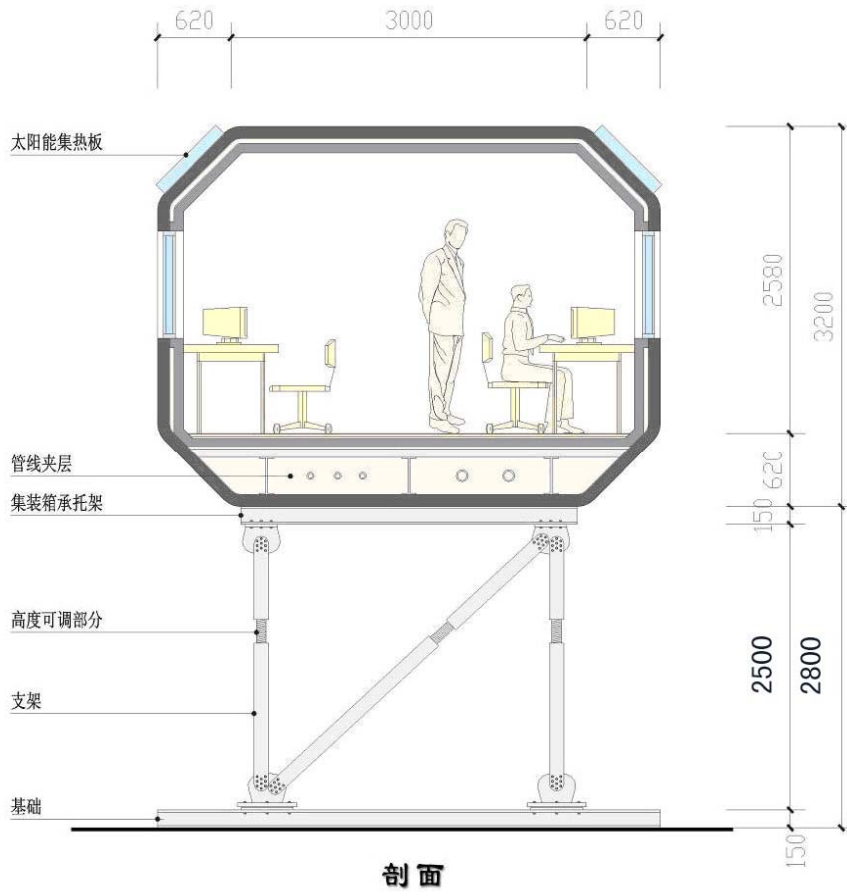
Fig. 19 Sectional drawing of deformed container
