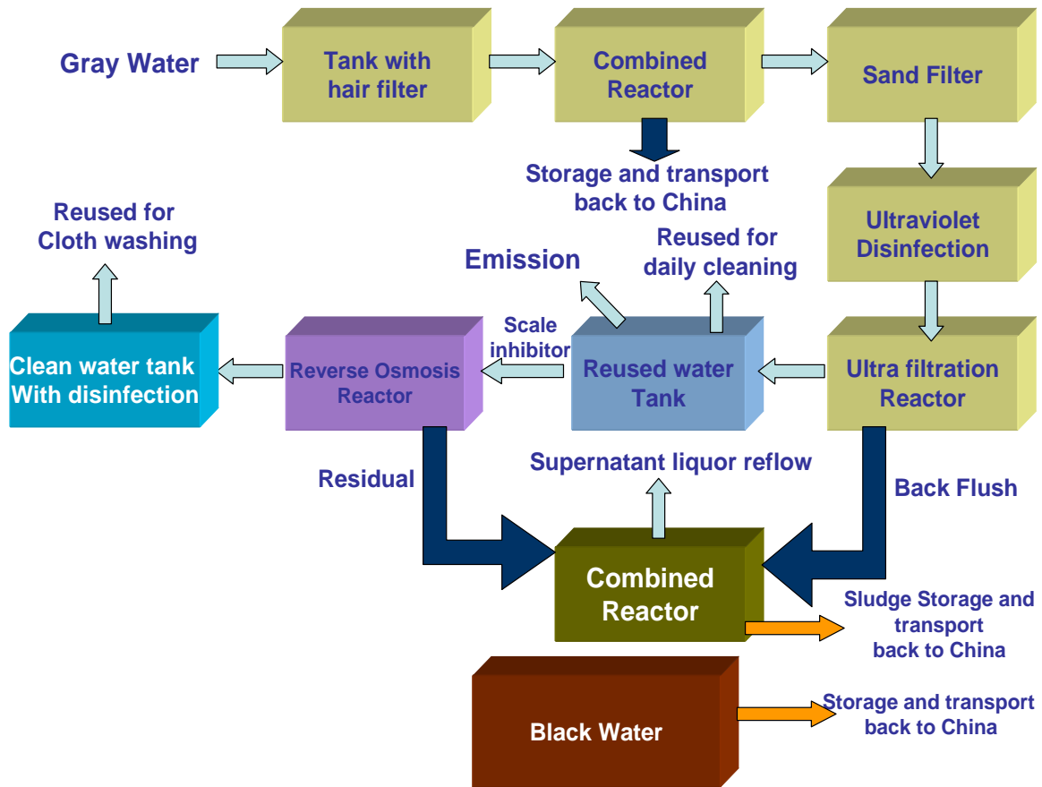
Fig. 23 Techniques for sewage treatment and recycling system
