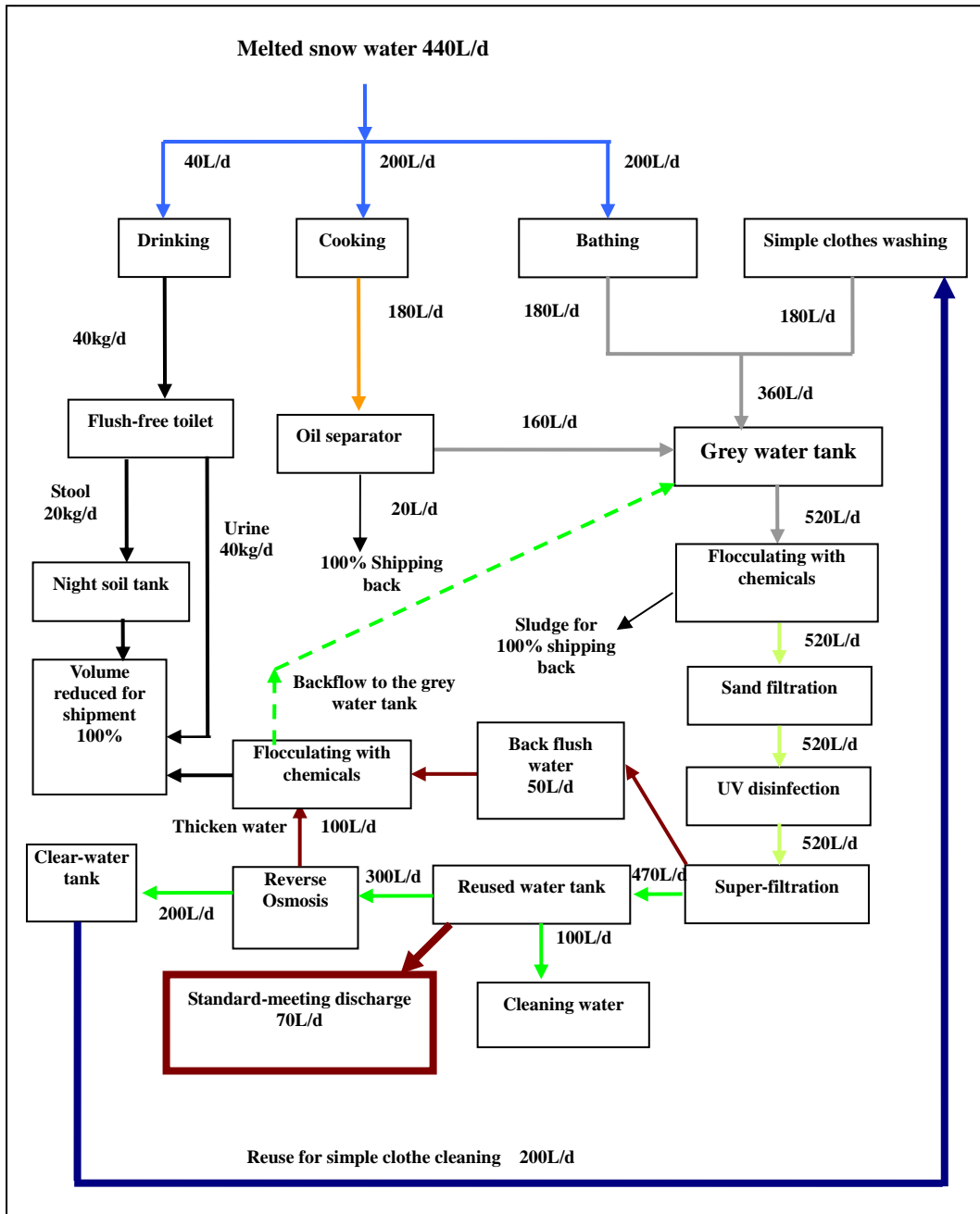
Fig. 22 Water balance and technological process in the Dome A Station
